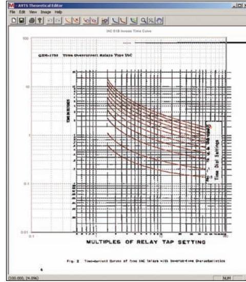
Westinghouse CO-9 Digitized Time-Current Curves
